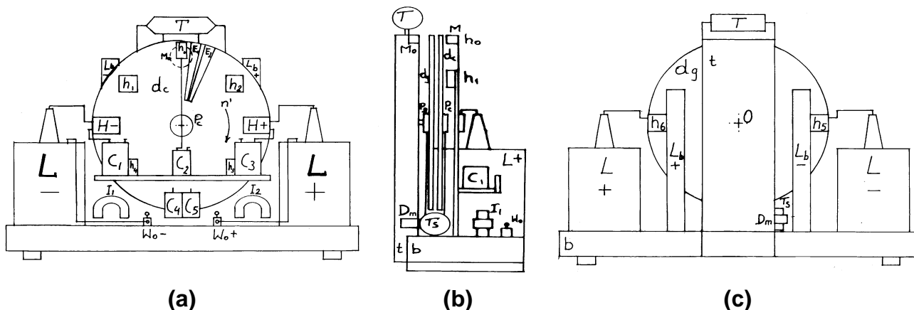
Fig. #F1abc (LA5 in [1/5]): The mechanical design and main components of the telekinetic INFLUENZMASCHINE. Because my original drawings of this machine were lost, the above illustration represents only their reconstruction from my memory, supported with descriptions quoted in subsection LA2.3.3 of [1/5] that were saved in my personal computer. The dimensioning of drawings was done in an approximate manner, means without using any scale. (Click on any above drawing to see it enlarged, or to shift it to another area of the screen.)
