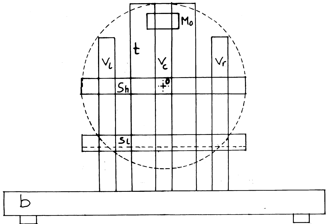
Fig. #F2 (LA5c in [1/5]): Carrying structure (frame) of the telekinetic influenzmaschine. To this frame components of telekinetic influenzmaschine are later assembled. (Click on the above drawing to see it enlarged, or to shift it to another area of the screen.)
