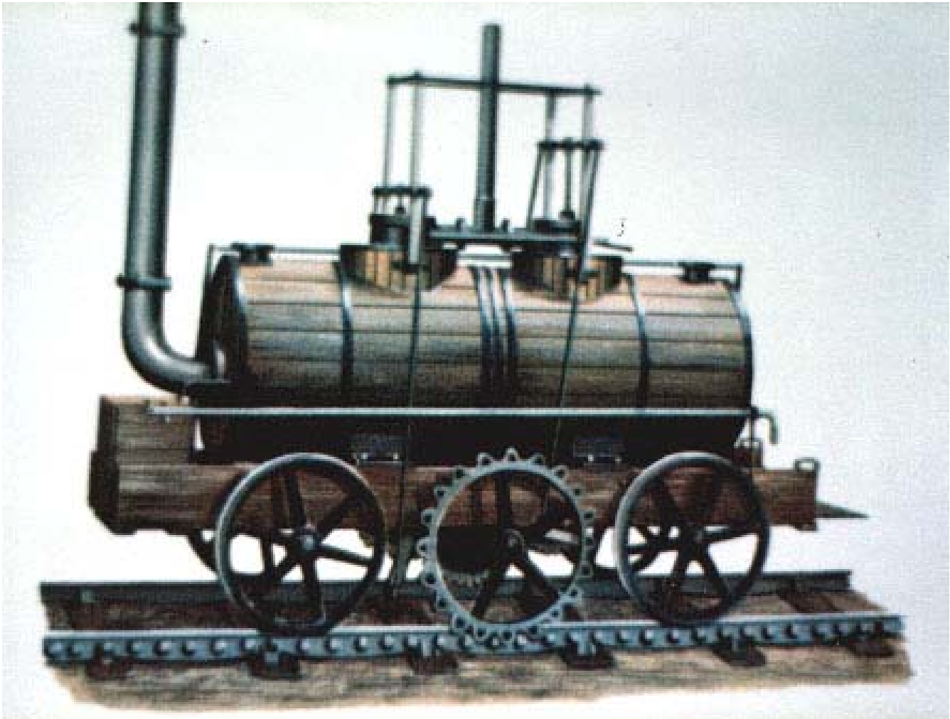
Fig. JB1. Blenkinsop's engine built in 1811. As the illustration shows, this locomotive was propelled by a pinion wheel winched along a cast-iron rack rail. The experts of that time were so used to thinking in terms of horse-power and horse legs, that they totally rejected and derided Hedley's solution to the adhesion problem, that led to the idea of propelling a train by smooth iron wheels that are rolled along smooth iron rails. They believed that such smooth iron wheels must slip on smooth iron rails, thus rotating in the same spot and not being able to haul a heavy train. Therefore, if this young creator had not been lucky enough to find the authoritative sponsor who financed his revolutionary invention, locomotives would probably still be using a solution similar to this illustration. Perhaps if this had not happened, our contemporary cars would also be running with legs like horses. Because of William Hedley our civilization won this battle with close-minded people. But no-one knows in how many other areas conservatism has predominated, so that "horse-type" solutions still hold sway.
